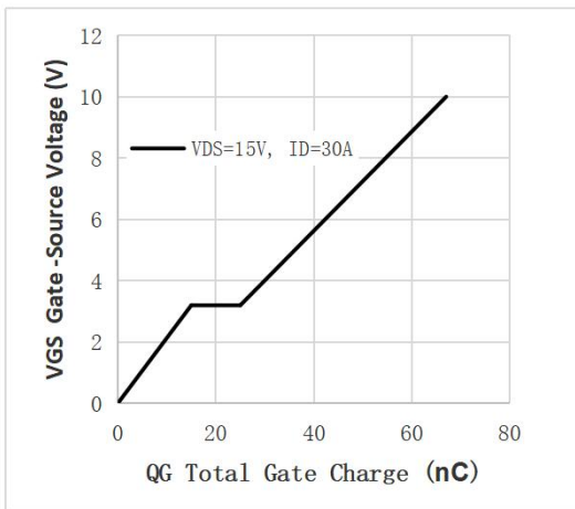
Fig.1 Gate-Charge Characteristics
