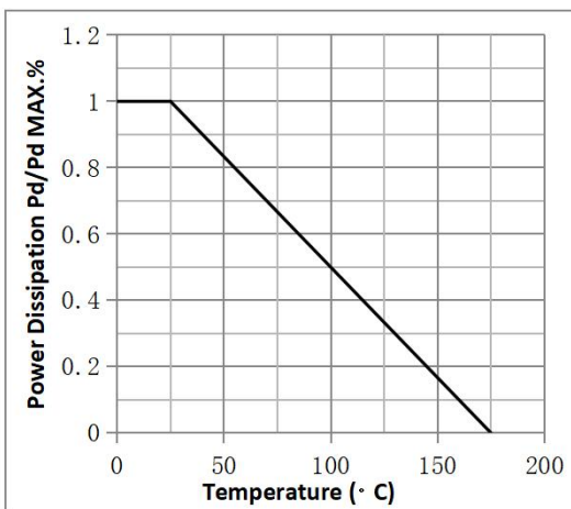
Fig.3 Power Dissipation
