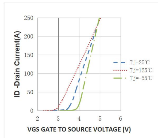
Figure 10. Transfer Characteristics
