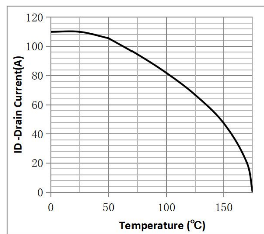
Fig.12 ID vs. Case Temperature ®
