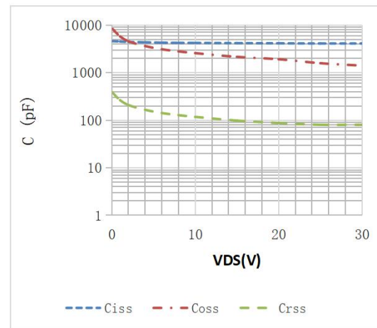
Fig.2 Capacitance Characteristics
